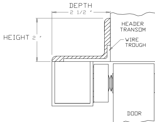
1194 ANGLE BRACKET
