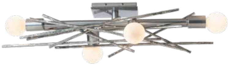
NEW BRINDILLE 4-LIGHT LARGE SCIONCE/SEMI-FLUSH 212034 - 10.1" h x 35" w x 7.9" d - 12 lbs - 5" x 7" backplate 4.7" vertical mounting ht - 16.5" horizontal mounting ht medium sockets (4), 15 watt max, G25 bulbs, incl Note: Can hang vertically, horizontally, or as a semi-flush
