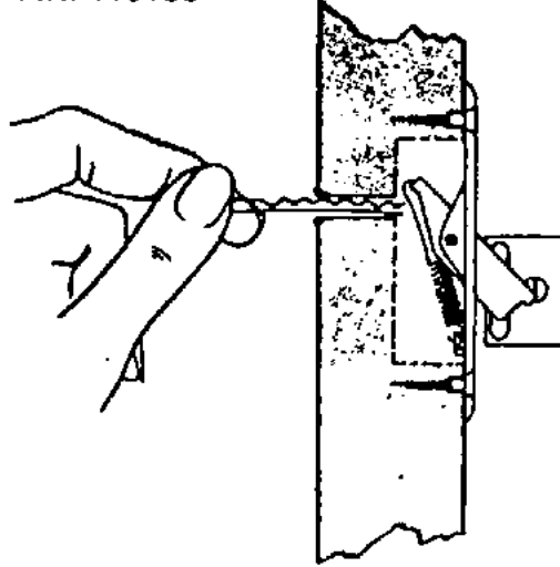
COMPLETED INSTALLATION IVES No. 42 JAMB BOLT
