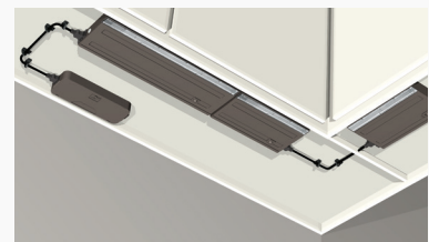
Front Mount – Use wire module and interconnect cable.
