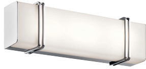
45801CHLED | Impello™ Chrome | Satin Etched White (1), 20W, 900lm, 3000K, 90 CRI, 45 LPW 18.25"W x 5.5"H | Ext. 3.5"
