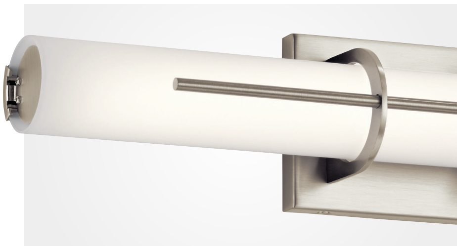
83759 | Rowan Brushed Nickel | Etched Opal Glass (1), 42W, 2400lm, 3000K, 90 CRI, 57 LPW 25.25"W x 4.75"H | Ext. 3.13"
