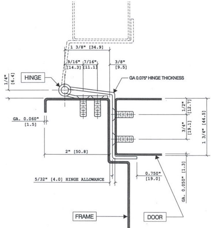
SWING CLEAR HINGE GUARD
