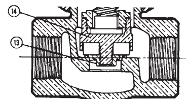
T-275-Y
