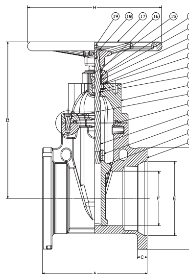
MJ-619-RWS
