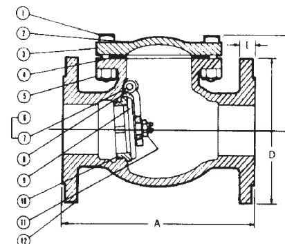
F-938-33
