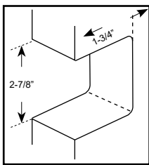
Notching Dimensions
