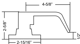
Latch: 1"x2-1/4" round corner, adjustable backset, UL Strike: FT4SPG: 1-3/4"x2-1/4" full lip strike, round corner
