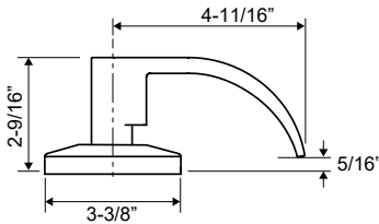
Latch: 1-1/8"x2-1/4" square corner, 2-3/4" backset, UL Strike: FASA: 1-1/4"x4-7/8", square corner
