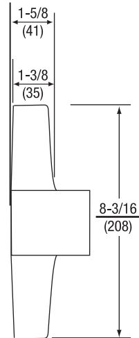
Cover Detail
