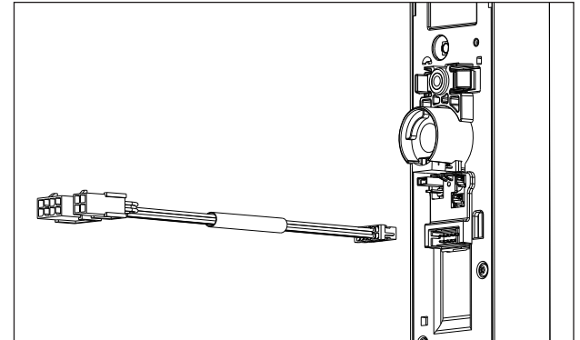
Diagram 5 Connect Lock Interface Cable (B)
