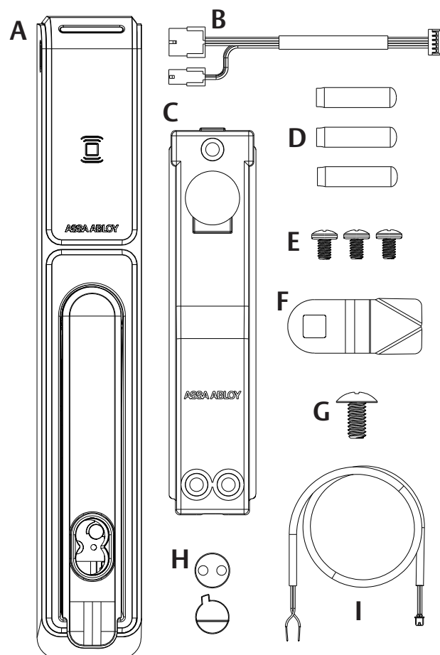
Diagram 1: Product Components
