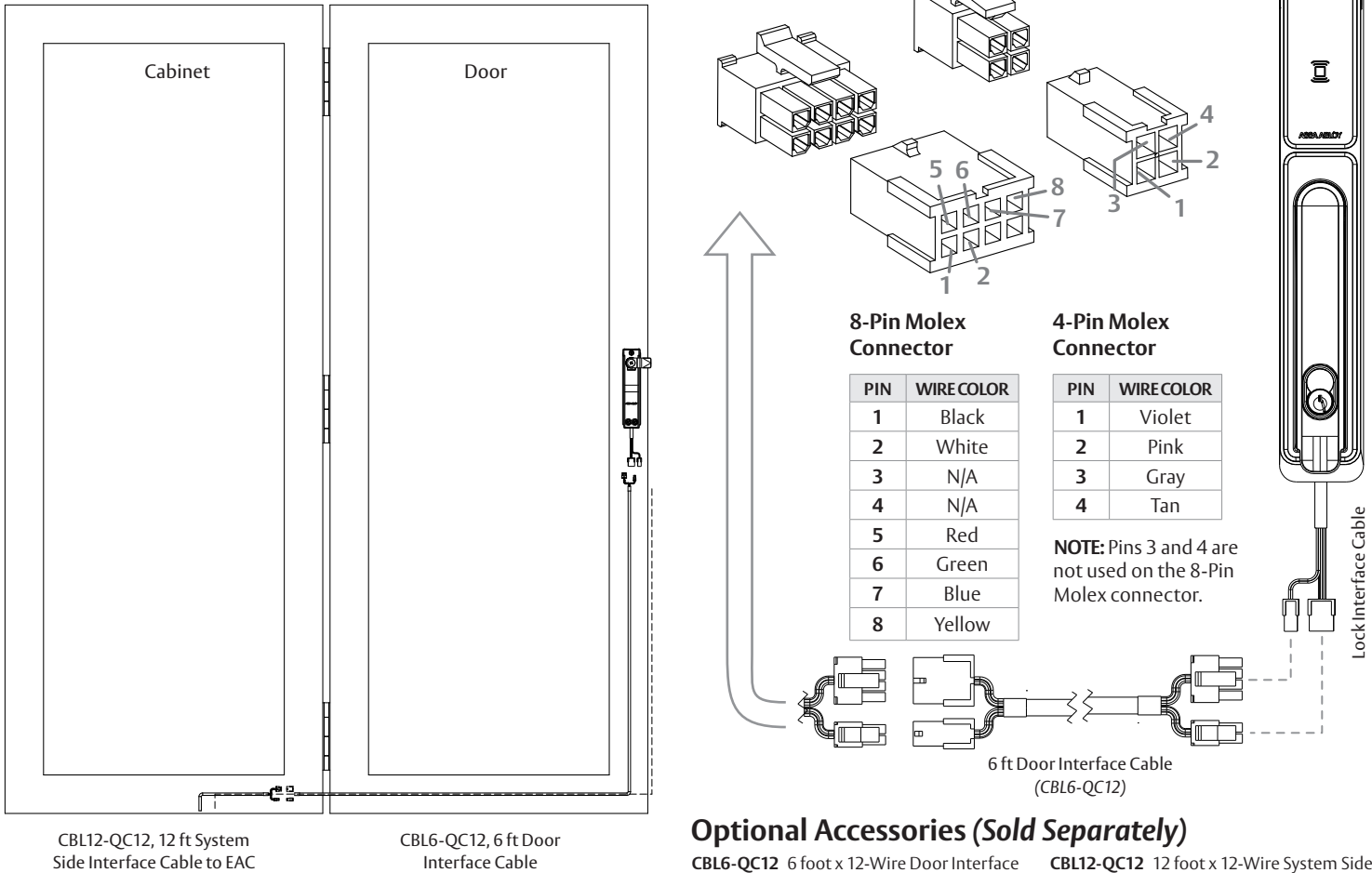
Diagram 12 Server Cabinet Wiring Example
