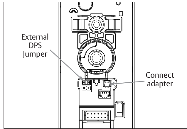
Diagram 7 DPS Activation
