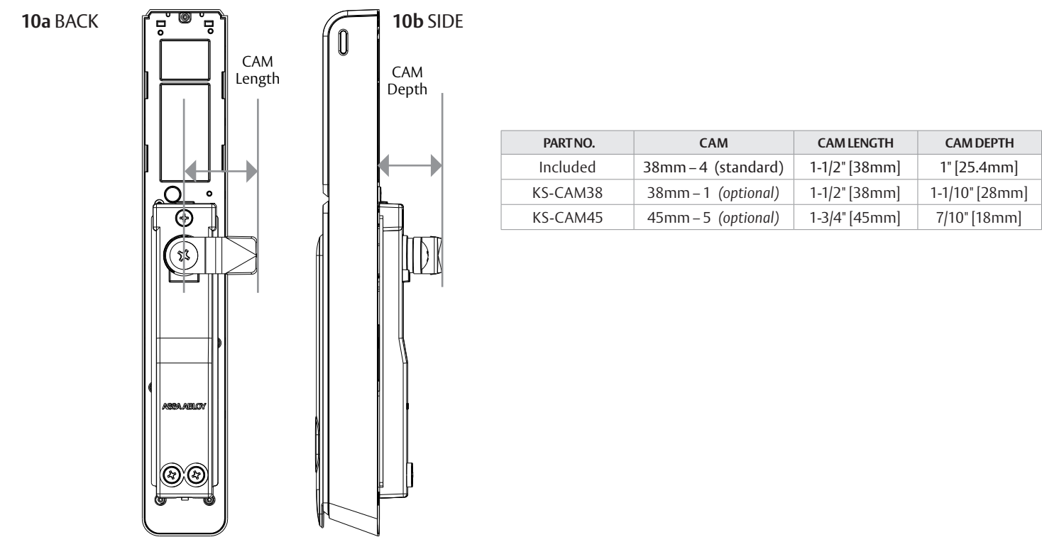
Diagram 10 KS Cam Length Selection
