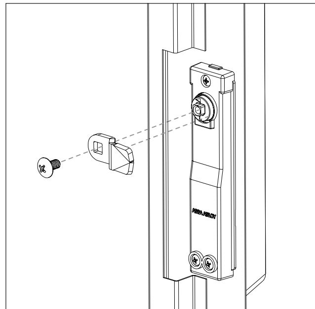
Diagram 9 Install Locking Cam (F) with Truss Head Screw (G)
