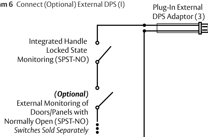
Diagram 6 Connect (Optional) External DPS (I)
