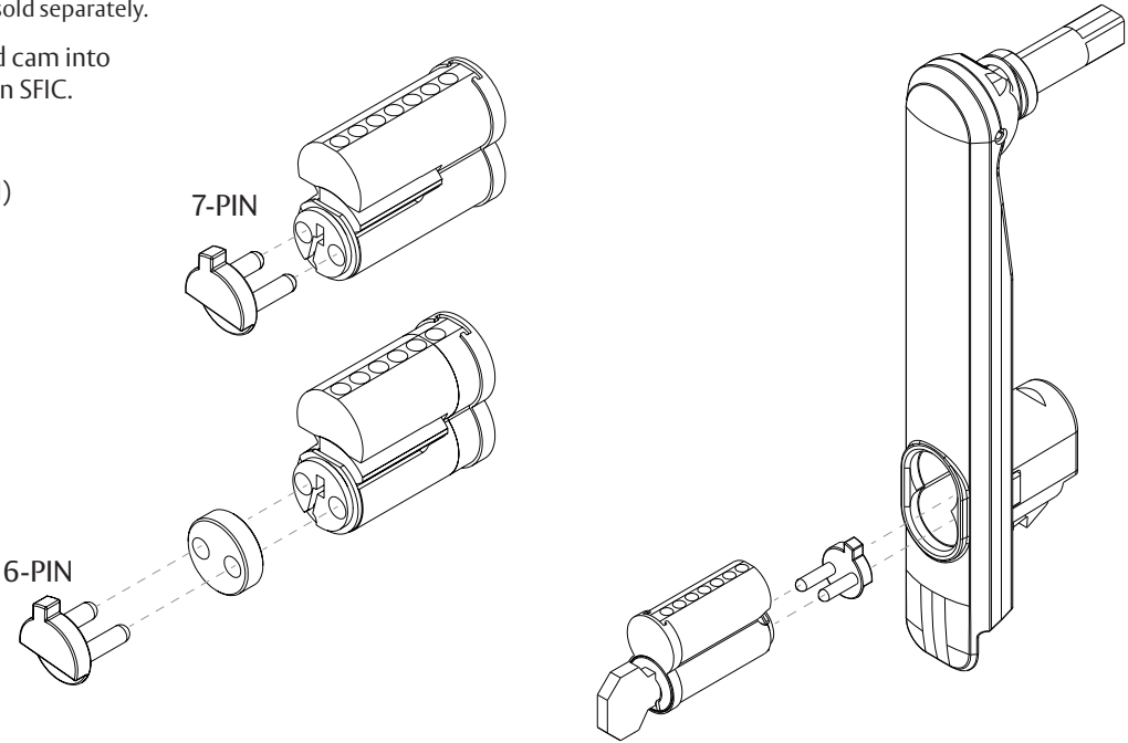
Diagram 11 6 or 7-pin SFIC (H)
