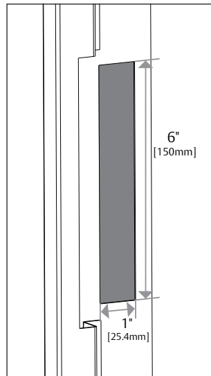
Diagram 2 Door Preparation
