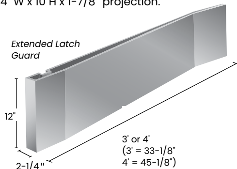
Latch Guard
