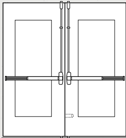
Two surface mounted vertical rod devices, less bottom rod (LBR). For LBR fire device, auxiliary fire pin is required.*
