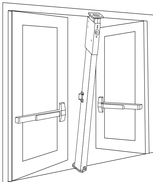
Keyed removable steel mullions
