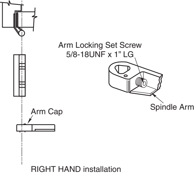
RIGHT HAND installation
