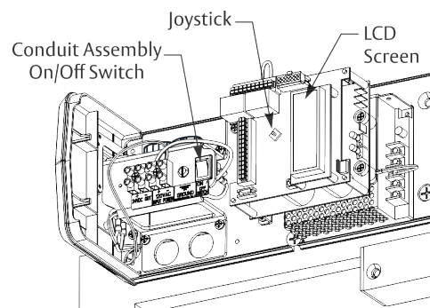
Figure 27 Union Assembly and Spacer not shown
