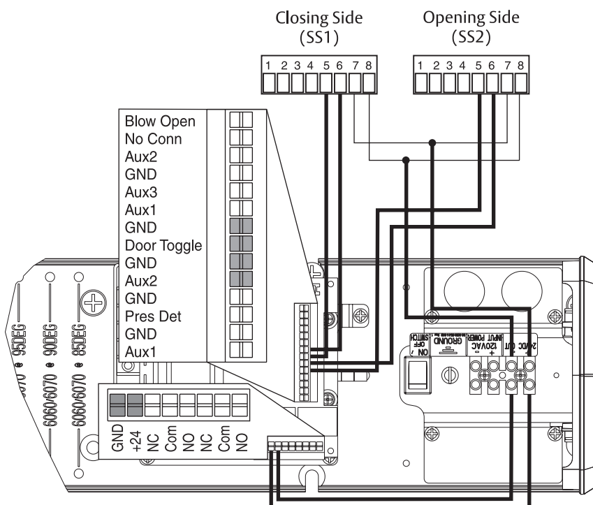
Door Mounted Presence Sensor
