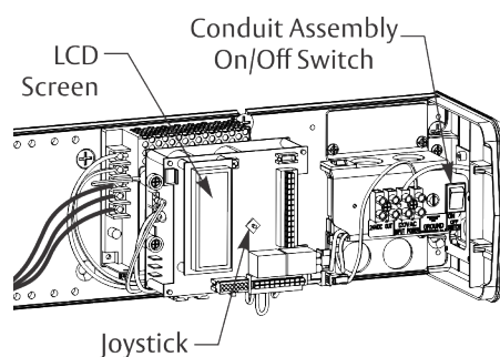
Figure 27 Union Assembly and Spacer not shown
