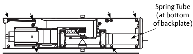
Figure 12 Remaining LAP Mounting Screws - Left Hand View
