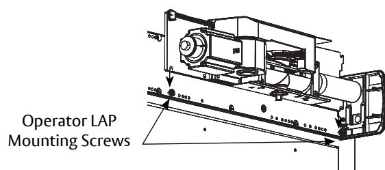
Figure 11 Left Hand LAP shown
