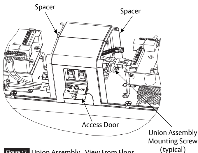
Figure 17 Union Assembly - View From Floor
