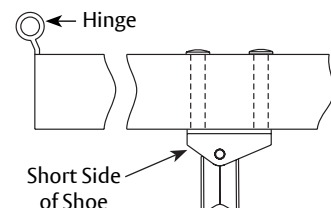
Figure 20 View from ceiling looking downward
