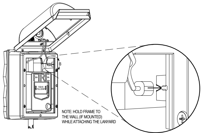
VIEW B
