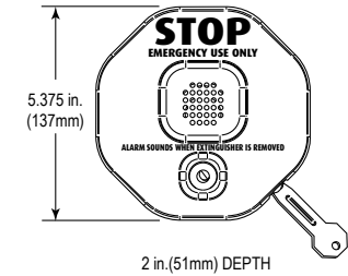
PRODUCT DIMENSIONS
