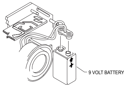
BATTERY REPLACEMENT
