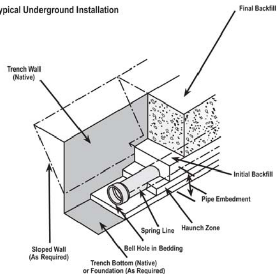
Typical Underground Installation
