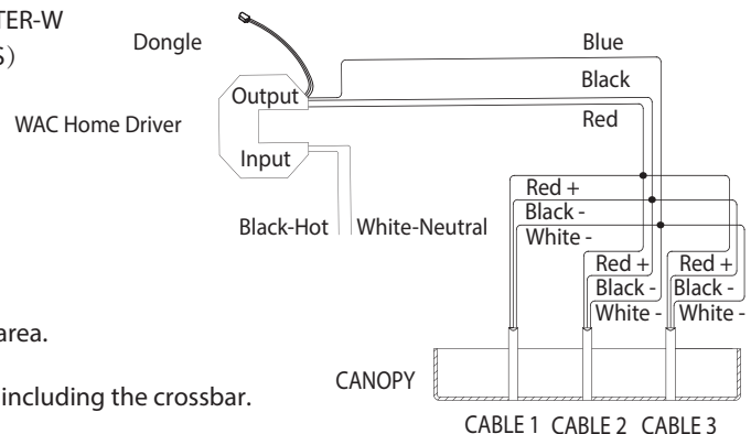
Fig.4 Driver Wires
