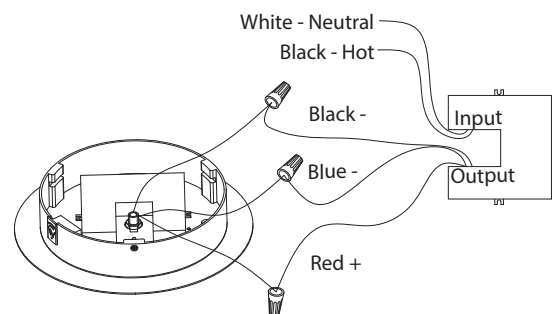
Fig. 3 Driver Wiring
