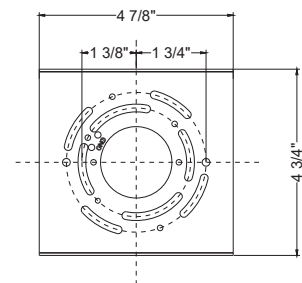
Mounting Plate Dimensions
