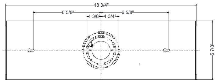
Mounting Plate Dimensions
