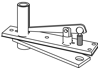
Extended Pin Walking Beam Pivot (PV-345)
