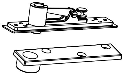
Walking Beam Pivot (PV-WALKBEAM)
