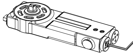
Overhead Closer (OHC-609)
