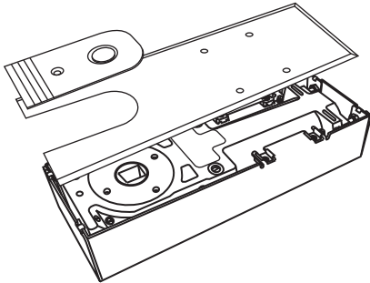
Standard Duty Floor Closer (FC-6275)
