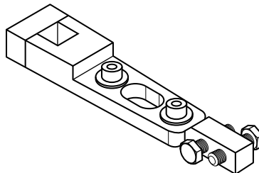
Overhead Closer and Bottom Pivot Arm (DOHC-275)
