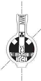
Change key inserted in cylinder.
