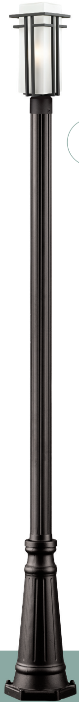
D. 550PHM-519P-ORBZ W:10" H:111" Cut post to suit desired height 1-100w/m
